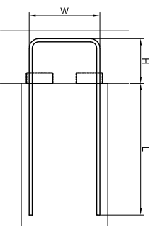
FERBOX SHAPE 21D
