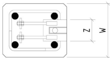
Figure A2-2: Illustration - minimum column width to allow for space of the unit
