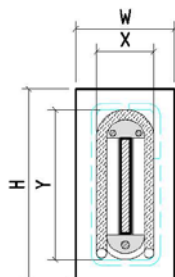
Figure A2-1: Illustration - evaluation of minimum beam dimension to allow for space of the unit
