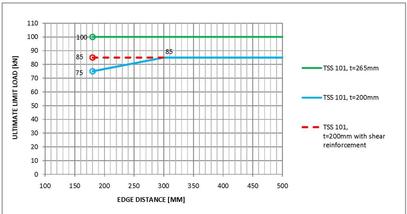
Figure 3: Recommended ultimate limit load when using TSS 101 with slab thicknesses t = 200\text{mm} - 265\text{mm} .
