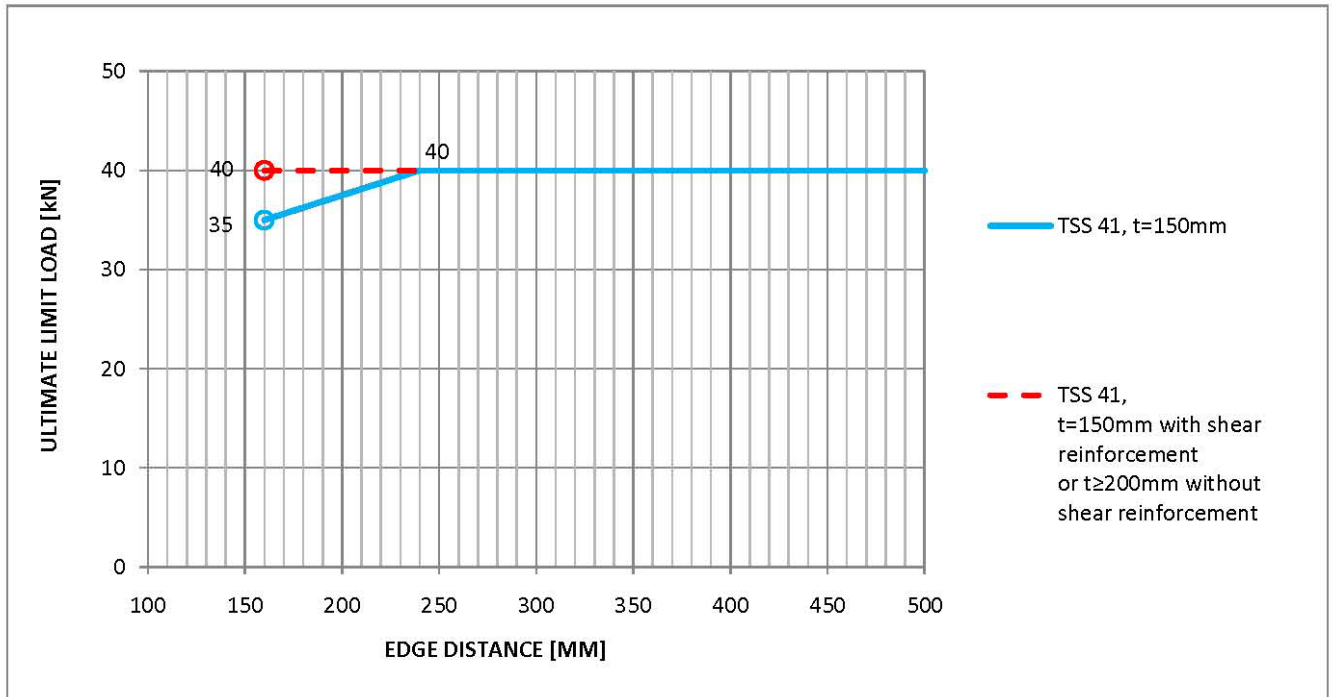
Figure 2: Recommended ultimate limit load when using TSS 41 with slab thicknesses t \geq 150\text{mm} .
